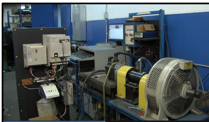
Eddy Current Load Stand
